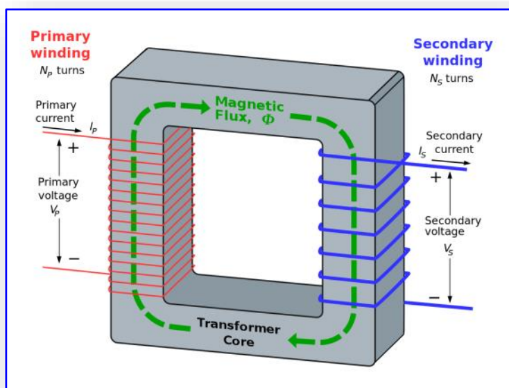
Schematic drawing of an AC transformer
