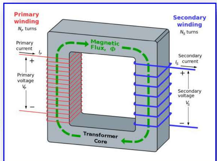
Schematic drawing of an AC transformer
