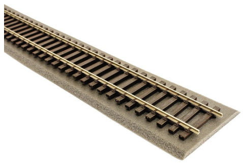
DCU-TBH3 100ft (31m) of super-high quality OO/HO scale trackbed.
